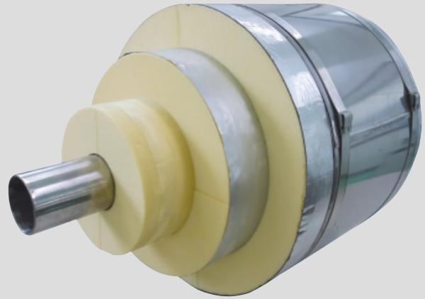
PIR/PUR pipe cover with SUS jacketing
