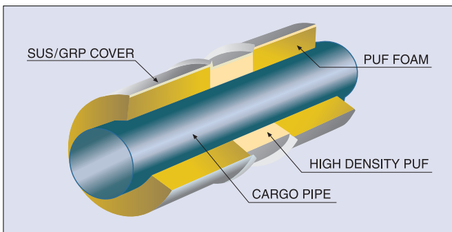
Insulation Construction
